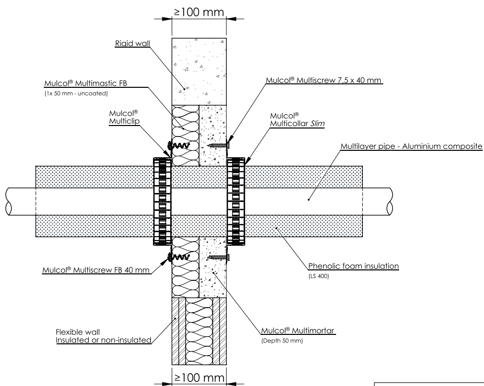
Drawing: FW.E-MLA-MM2.5.10
